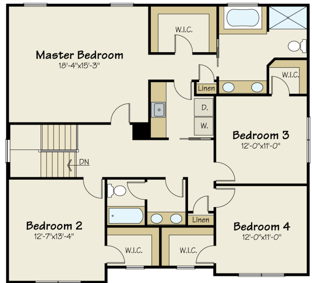
Elevation A & B Second Floor (note elevation B has no windows in closets)
